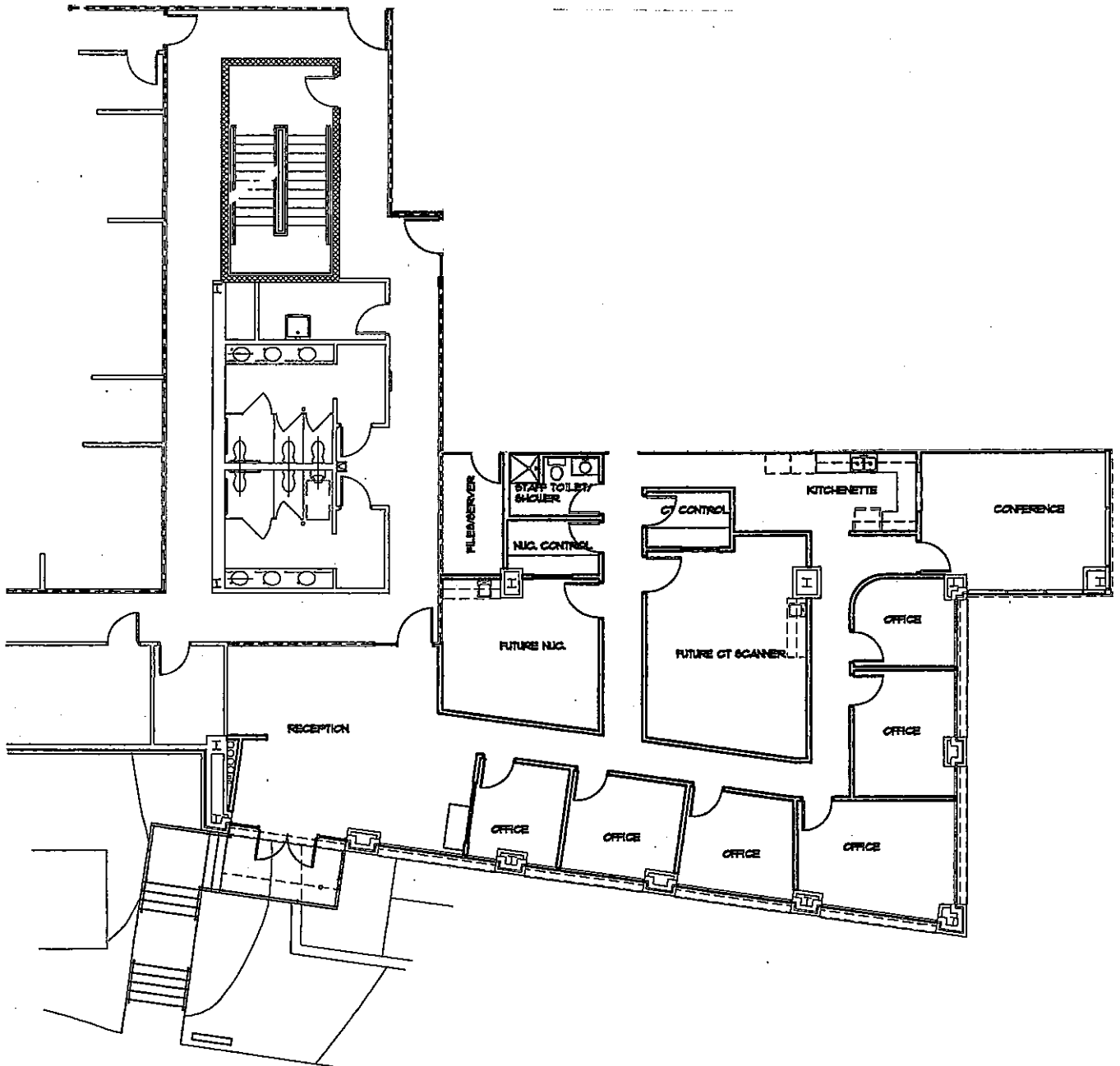
1 FLOOR PLAN A2.1 1/16"=1'-0"
