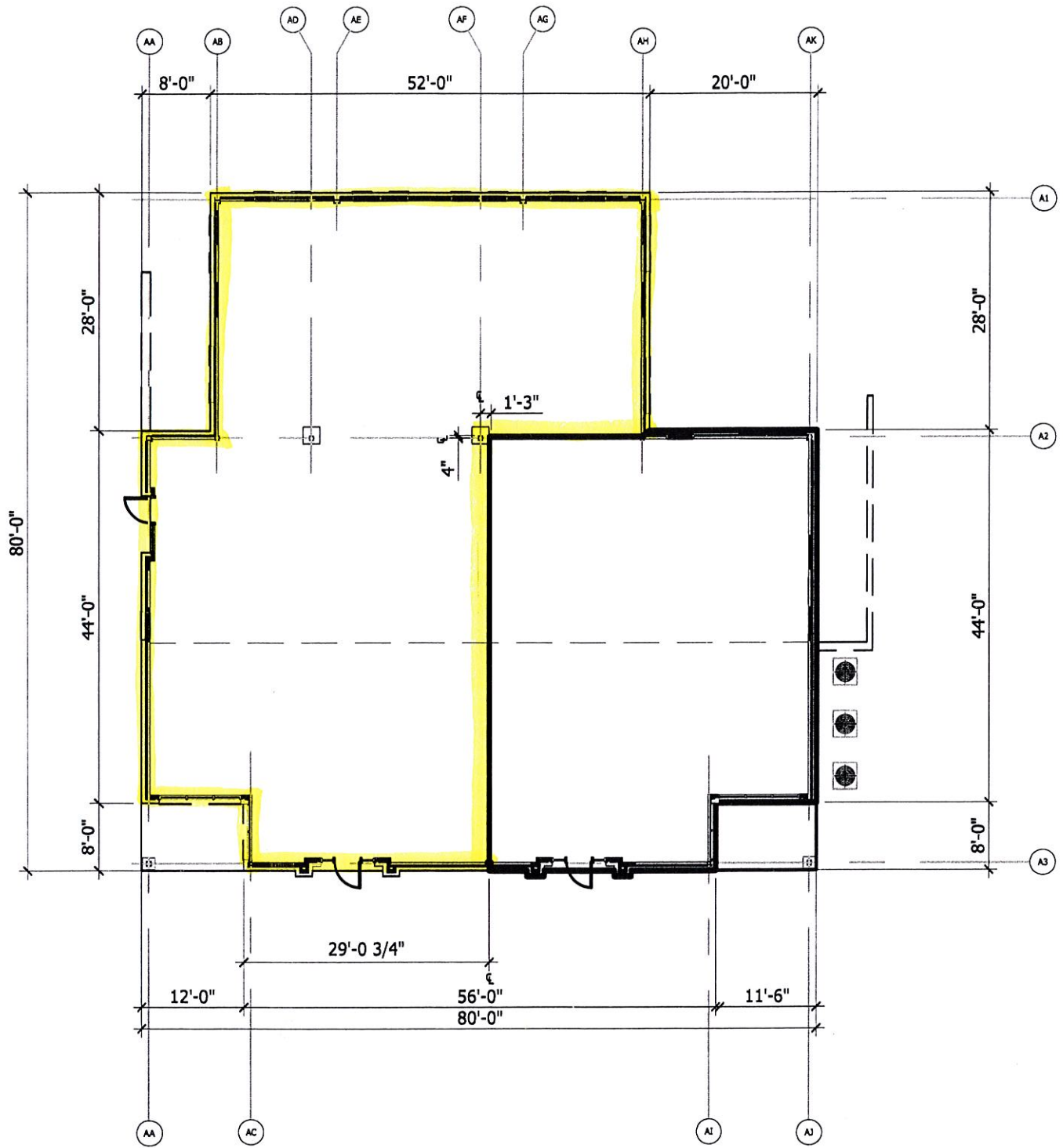
1 UPPER LEVEL PLAN - BLDG. A NTS
